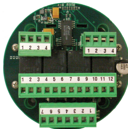
SEC 3120 Termination Board
